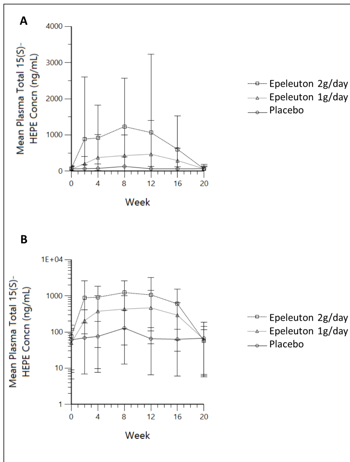
A. Mean plasma total 15(S)-HEPE concentrations (ng/mL) versus time (linear scale). B. Mean plasma total 15(S)-HEPE concentrations (ng/mL) versus time (semi-logarithmic scale). 15(S)-HEPE indicates 15-hydroxy eicosapentaenoic acid and SD, standard deviation.
