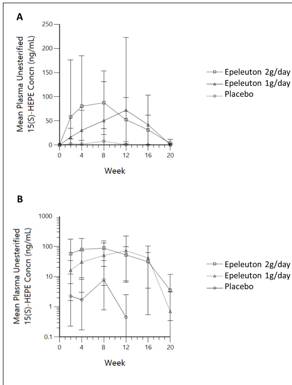
Figure S9. Mean ( \pm SD) plasma unesterified 15(S)-HEPE concentrations (ng/mL) versus time (linear and semilogarithmic scales) for epeleuton 1g/day, epeleuton 2g/day and placebo treated patients
